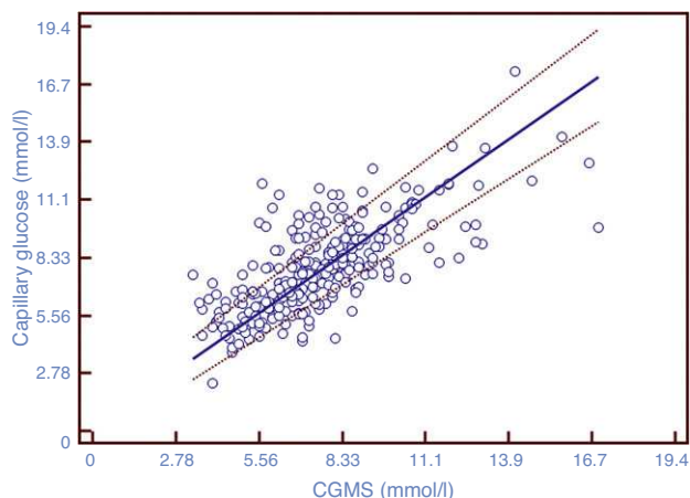
Figure 1 Scatterplot of paired data. The solid line represents the regression line; the dotted lines represent the confidence interval of 95%. Correlation coefficient = 0.71 ( p < 0.0001 ), 95% CI 0.65–0.76. The figure shows the existence of a positive linear correlation between the two methods of measurement.
